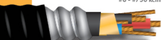
VFD Teck 90 with 3 Ground Wires Copper Shield
