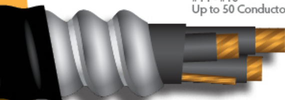
Large Teck 90 #1 - 600 kcmil Black Colour Coded Insulation
